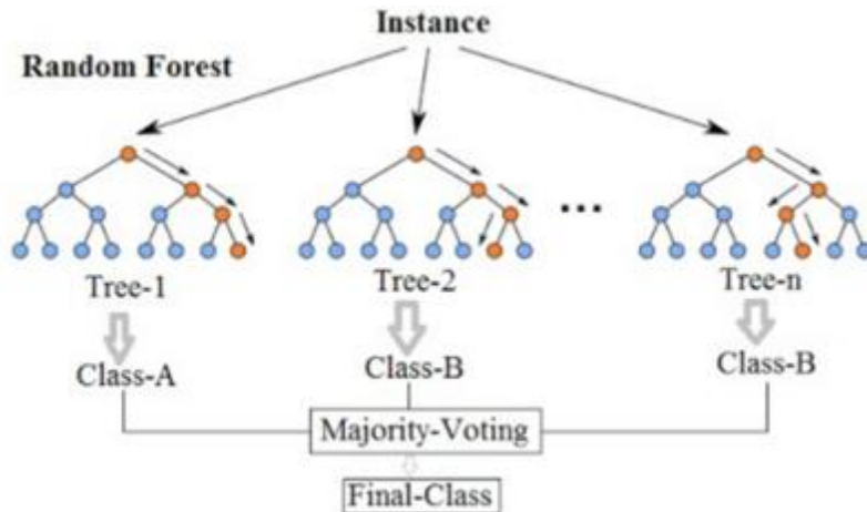
Random Forest
